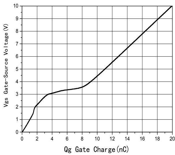
Fig6 Gate Charge
